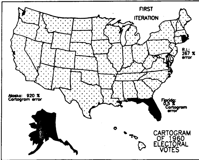
Figure 4. Selected proportionate error (after first iteration).
