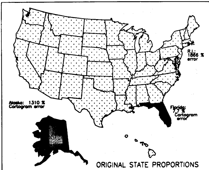
Figure 3. Selected proportionate error (equal area projection).
